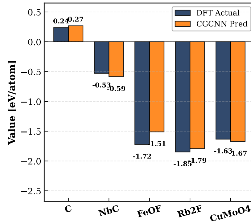
(b) Formation Energy ( E_f )
