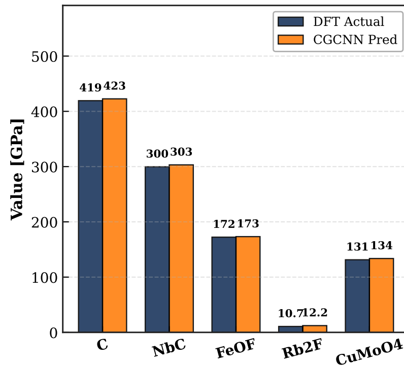
(e) Bulk Modulus ( K )
