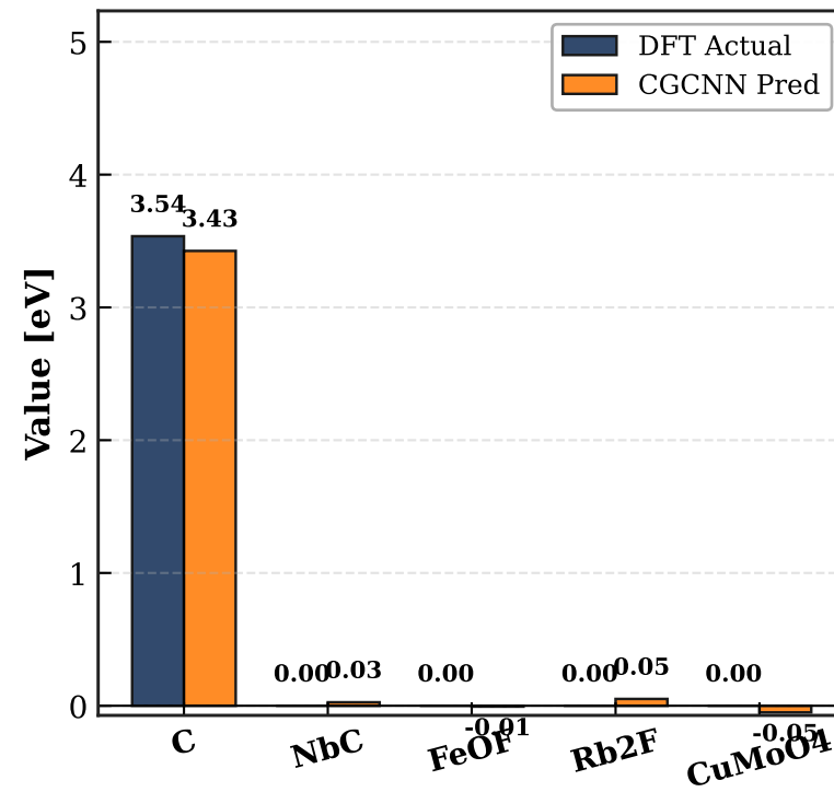
(a) Band Gap ( E_g )
