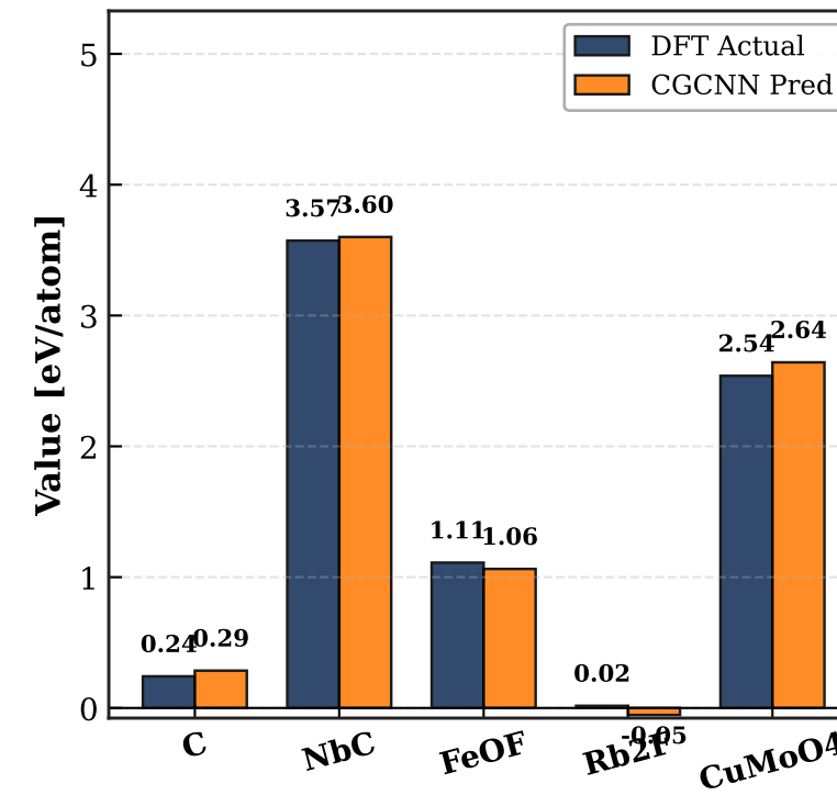
(c) Energy Above Hull ( E_{\text{hull}} )
