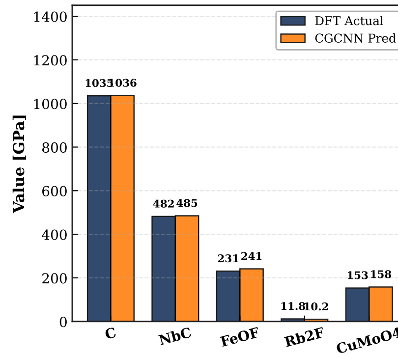
(g) Young's Modulus ( E )
