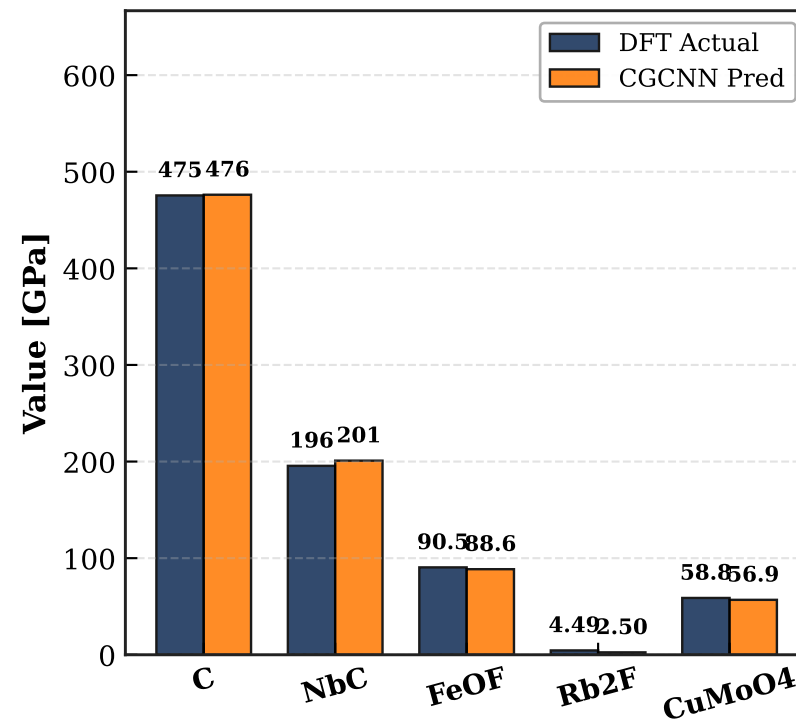
(f) Shear Modulus ( G )
